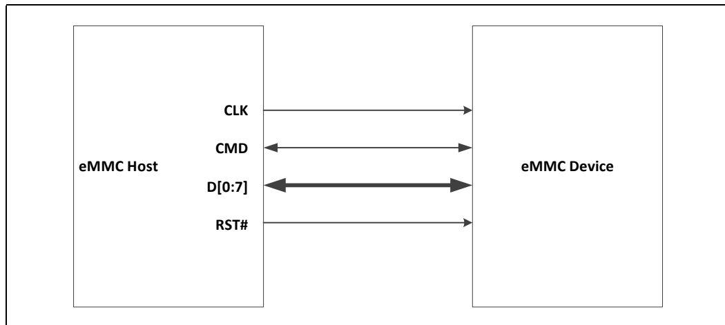
Figure 35. eMMC Interface
